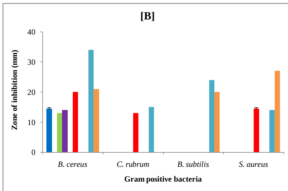
Figure 4:Zone of inhibition of Schiff bases against Gram positive bacteria in [A] DMF and [B] DMSO [SHA-1, (■); SHA-2, (■); SHA-3, (■); SHA-4, (■); SHA-5, (■); SHA-6, (■); SHA-7, (■); SHA-8, (■); Chloramphenicol (■); Tetracycline (■)]
