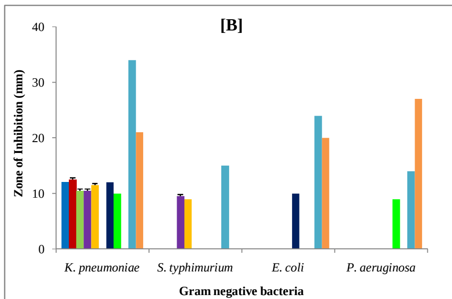
Figure 5:Zone of inhibition of Schiff basesagainst Gram negative bacteria in [A] DMF and [B] DMSO [SHA-1, (■); SHA-2, (■); SHA-3, (■); SHA-4, (■); SHA-5, (■); SHA-6, (■); SHA-7, (■); SHA-8, (■); Chloramphenicol (■); Tetracycline (■)]
