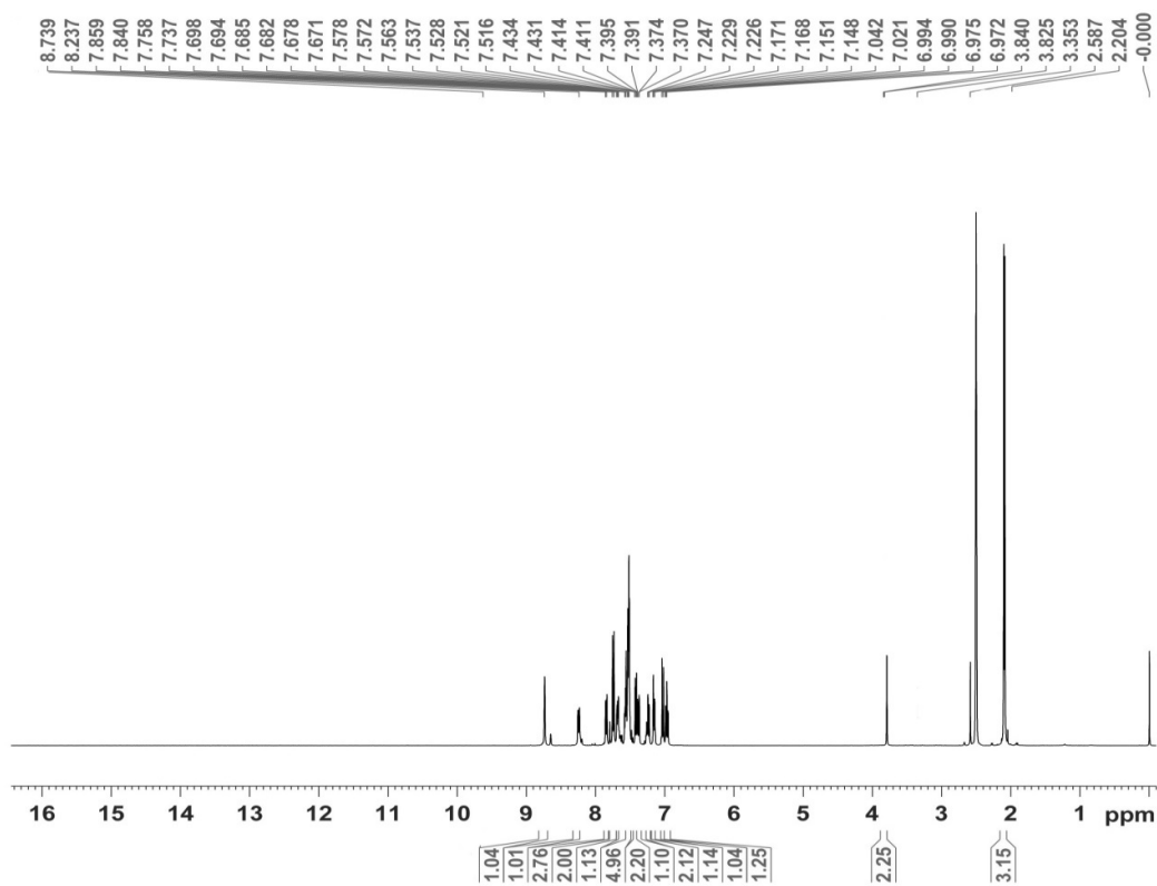
Figure-2: ^1\text{H} NMR spectrum of SHA-1
