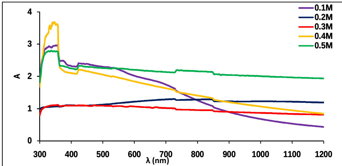
Figure 5. Absorbance spectra of variation in precursor concentration ZnO thin films.
