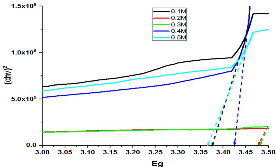
Figure 6. Plot of (\alpha h\nu)^2 \rightarrow h\nu , for ZnO multilayer thin films.
