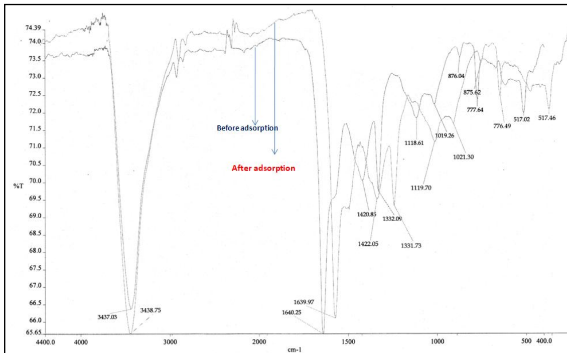
Figure 2: FT IR Spectra of carbon adsorbent sample before and after adsorption process
