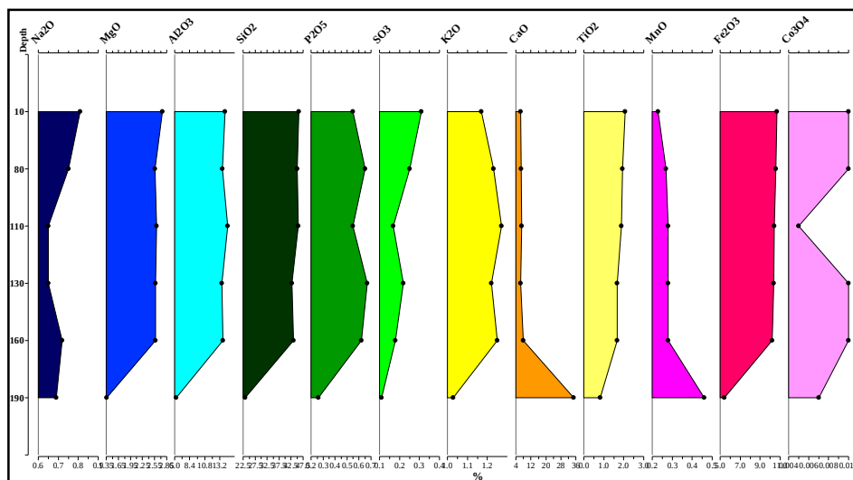
Fig. 5a: Profiles showing distribution of geochemical elements in section MS-B
