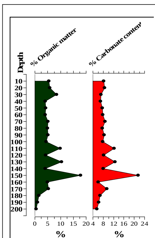
Fig. 6b Vertical profile of organic matter and Carbonate content in MS-B
