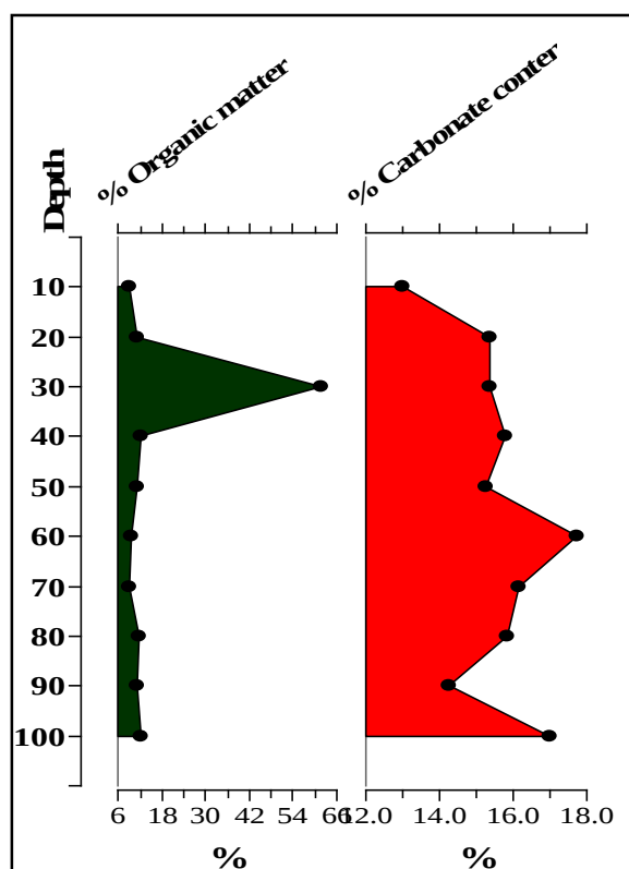
Fig. 6a Vertical profile of organic matter and Carbonate content in MS-A
