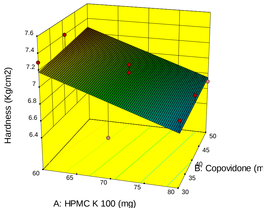
Fig 10: 3D plot for Hardness
