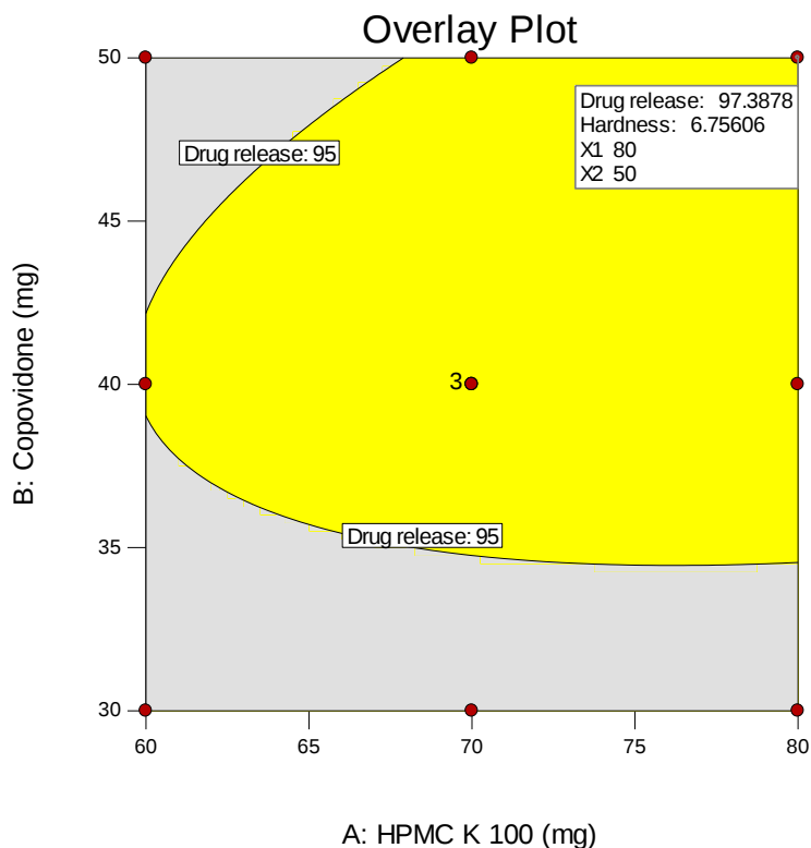
Fig 11: Overlay plot of all factors and responses
