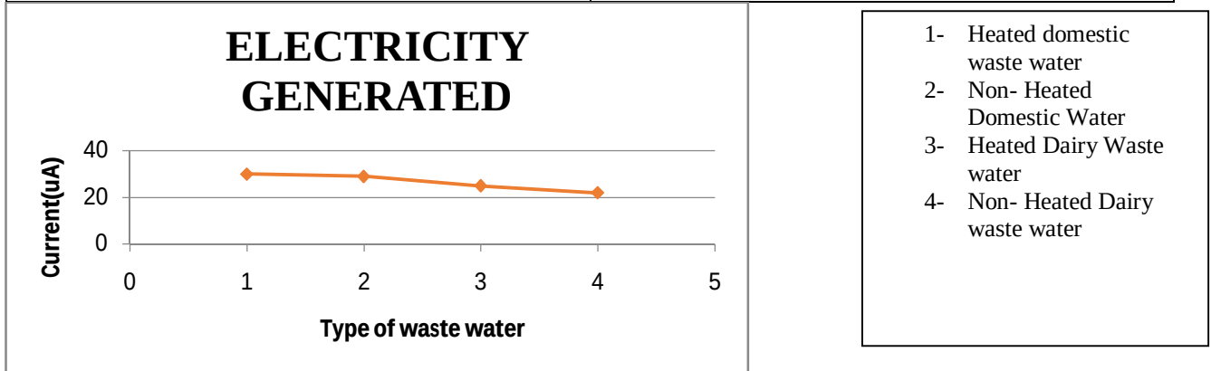
Figure 5.6 graph plotting electricity generation
