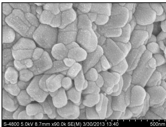
Figure 2 FESEM Photograph of \text{Sr}_2\text{CeO}_4: 0.5\%\text{Gd}^{3+}, 0.5\%\text{Eu}^{3+}
