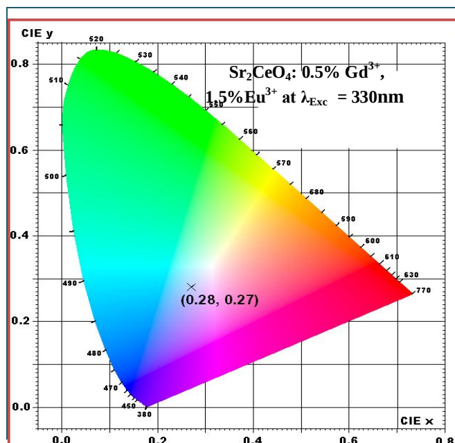
Figure 6 CIE Chromaticity diagram of \text{Sr}_2\text{CeO}_4: 0.5\% \text{Gd}^{3+}, 1.5\% \text{Eu}^{3+} at \lambda_{\text{Exc}} = 330 \text{ nm}
