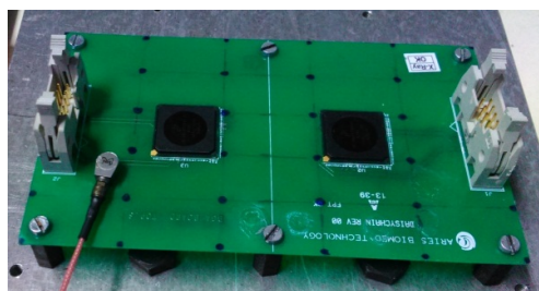
Figure 3 PCB divided into elements
