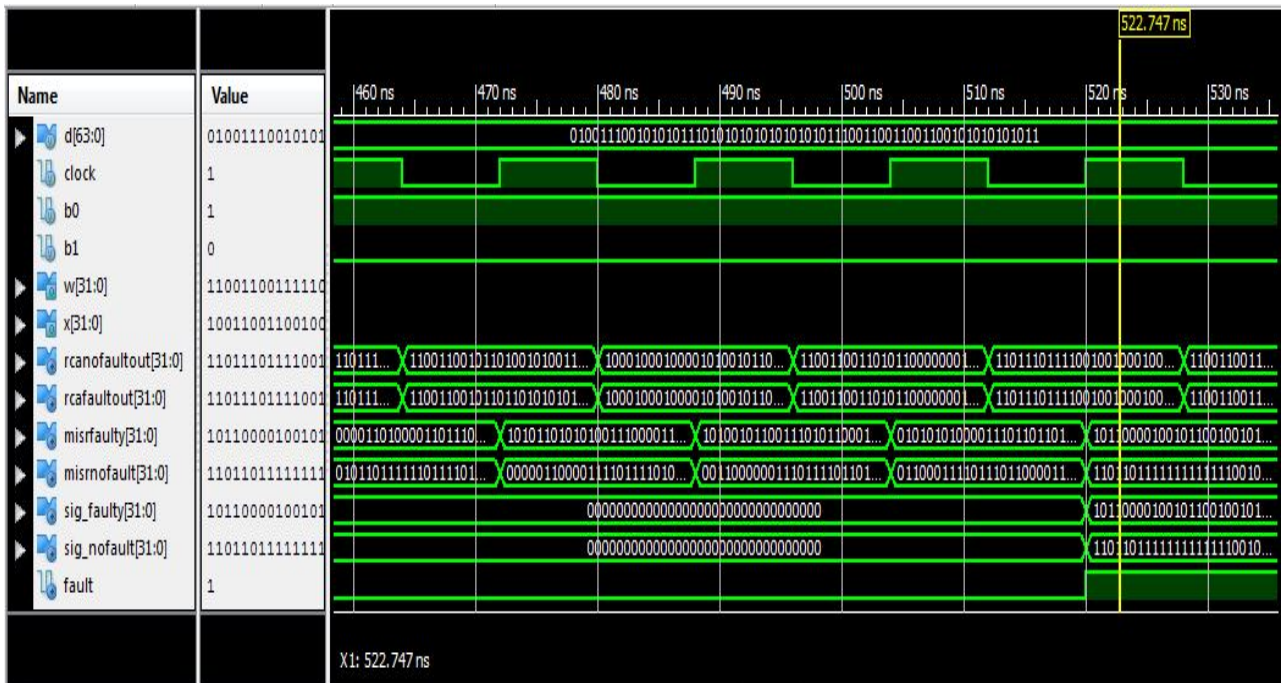
Figure 8: Simulation result of BILBO methodology for 32-bit Ripple carry adder
