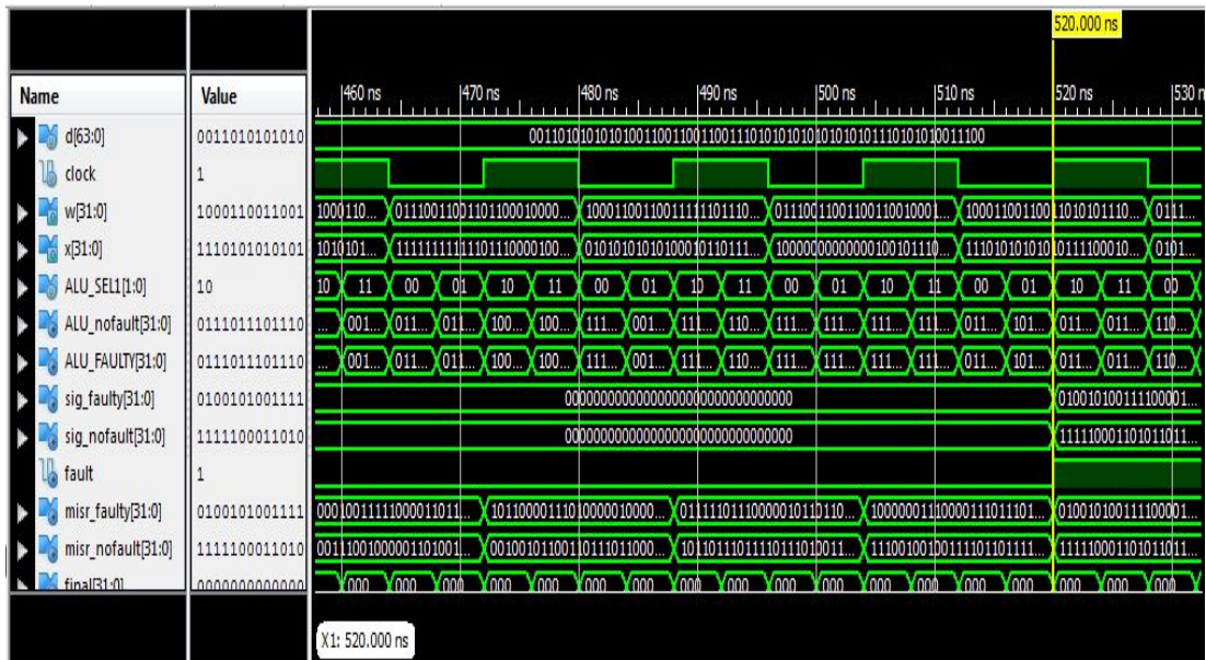
Figure 6: Simulation result of BILBO methodology for 32-bit ALU
