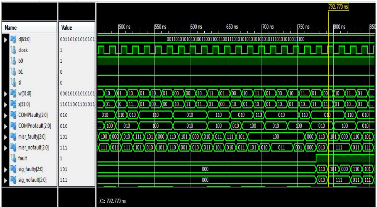
Figure 10: Simulation result of BILBO methodology for 32-bit magnitude comparator
