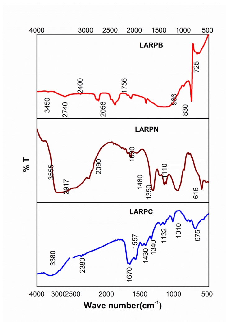
Figure 2. FT-IR spectra of L-arginine added crystals.
