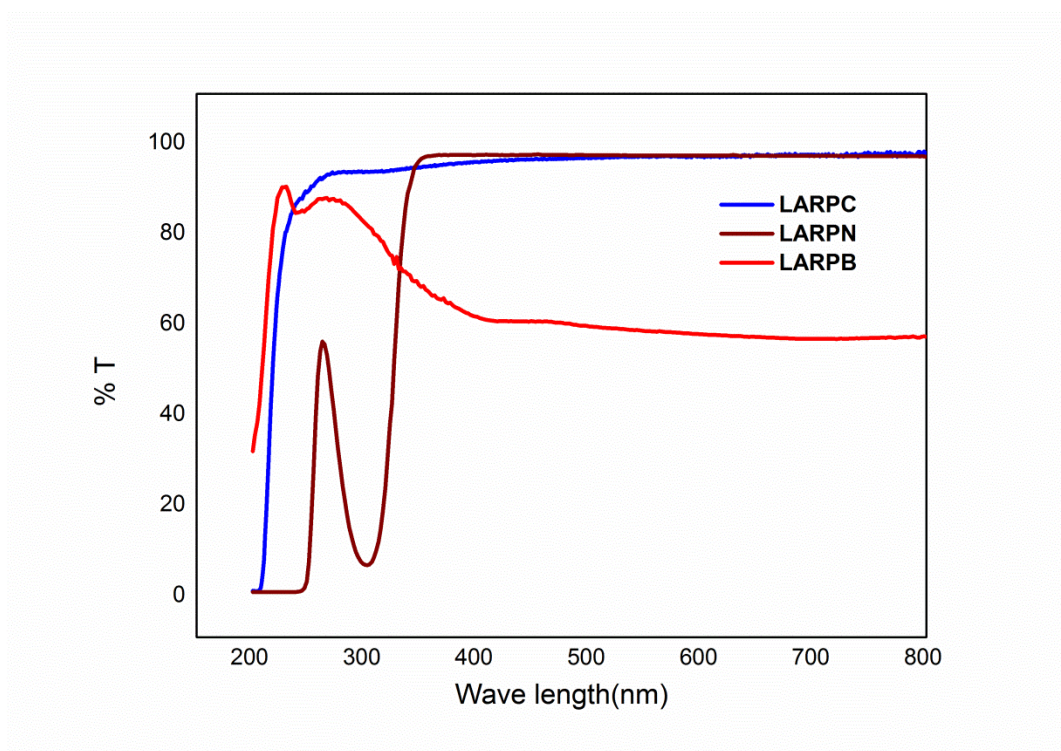
Figure 3. UV- visible spectra of L-arginine added crystals
