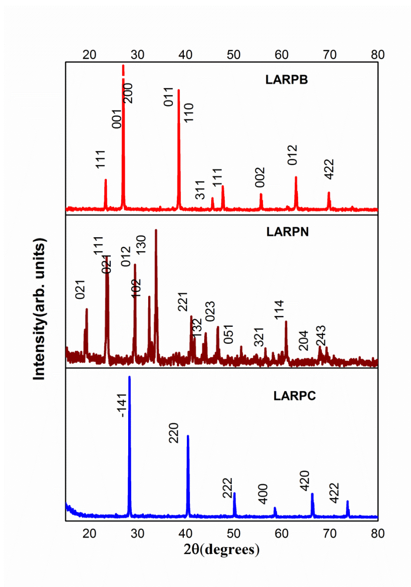
Figure 1. Powder XRD patterns of L-arginine added crystals
