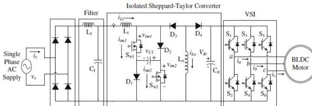
Figure 28. An Isolated Sheppard Taylor converter-fed BLDC motor drive 19
