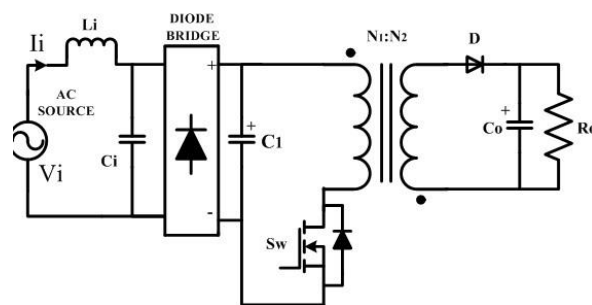
Figure 24. A Flyback converter 3
