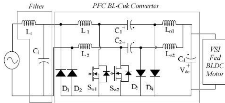
Figure 17. A Bridge-less Cuk converter-fed BLDC motor drive 1
