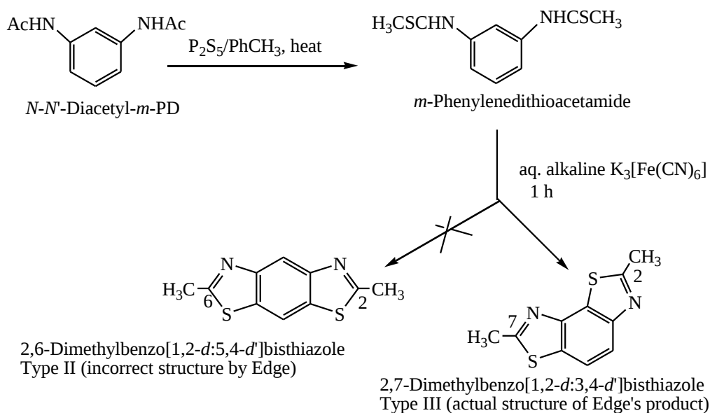
Scheme 9
