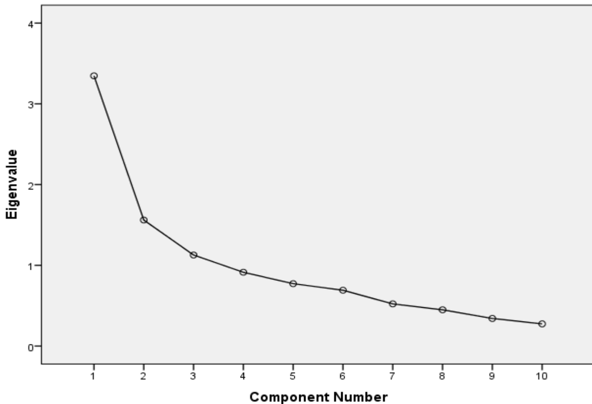
Scree Plot
