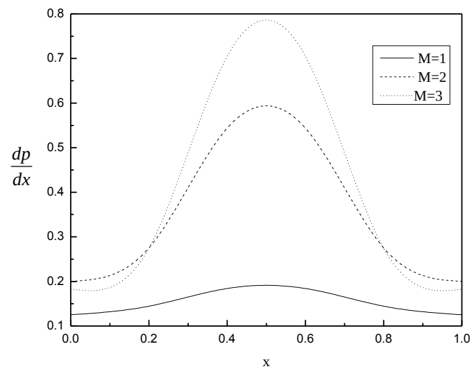
Fig. 3. The variation of axial pressure gradient with M for \phi = 0.6 , Da = 0.01 , \alpha = 0.1 , m = 2 , y_0 = 0.2 and \tau = 0.1
