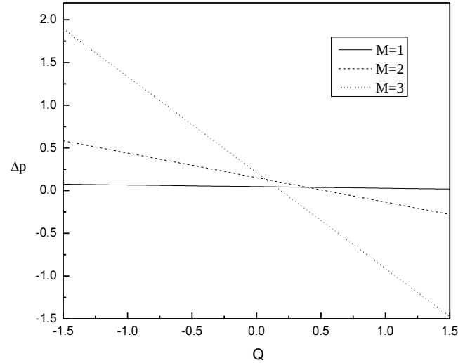
Fig. 10. The variation of pressure rise with time-averaged flux for different values M for \phi = 0.6 , Da = 0.01 , \alpha = 0.1 , m = 2 , y_0 = 0.2 and \tau = 0.1
