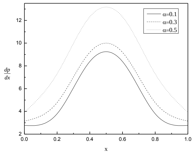
Fig.5. The variation of axial pressure gradient with \alpha for \phi = 0.6 , M = 2 , Da = 0.01 , m = 1 , y_0 = 0.2 and \tau = 0.01
