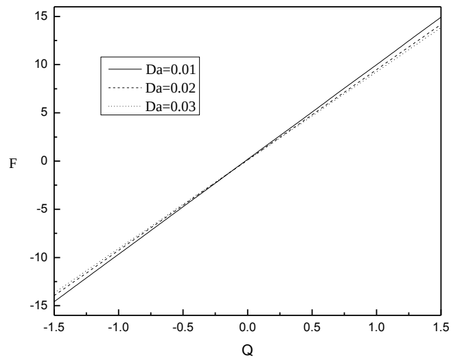
Fig. 12. The variation of frictional force with time-averaged flux for different values of Da for \phi = 0.6 , m = 1 , M = 4 , \alpha = 0.1 , y_0 = 0.2 and \tau = 0.01
