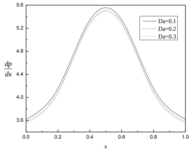
Fig.4. The variation of axial pressure gradient with Da for \phi = 0.6 , M = 4 , \alpha = 0.1 , m = 1 , y_0 = 0.2 and \tau = 0.01
