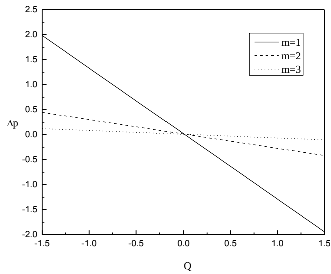
Fig. 6. The variation of pressure rise with time-averaged flux for different values m for \phi = 0.6 , Da = 0.01 , \alpha = 0.1 , M = 2 , y_0 = 0.2 and \tau = 0.01
