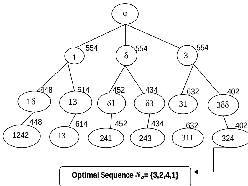
Fig.2: Scheduling Tree
